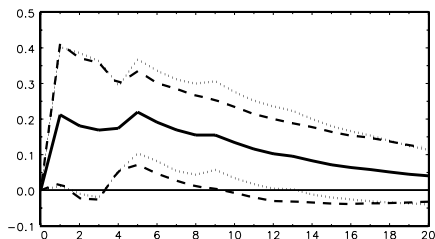
Figure 4.1. Forecast error impulse responses of German interest rate–inflation system based on subset VECM (3.41) (upper panel) and an unrestricted VAR(4) model (lower panel).
