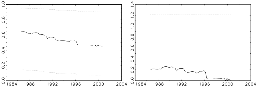
Figure 4.7. Recursive eigenvalue (left) and T -test with 10% critical value (right) of VECM with two lagged differences and r = 1 .
