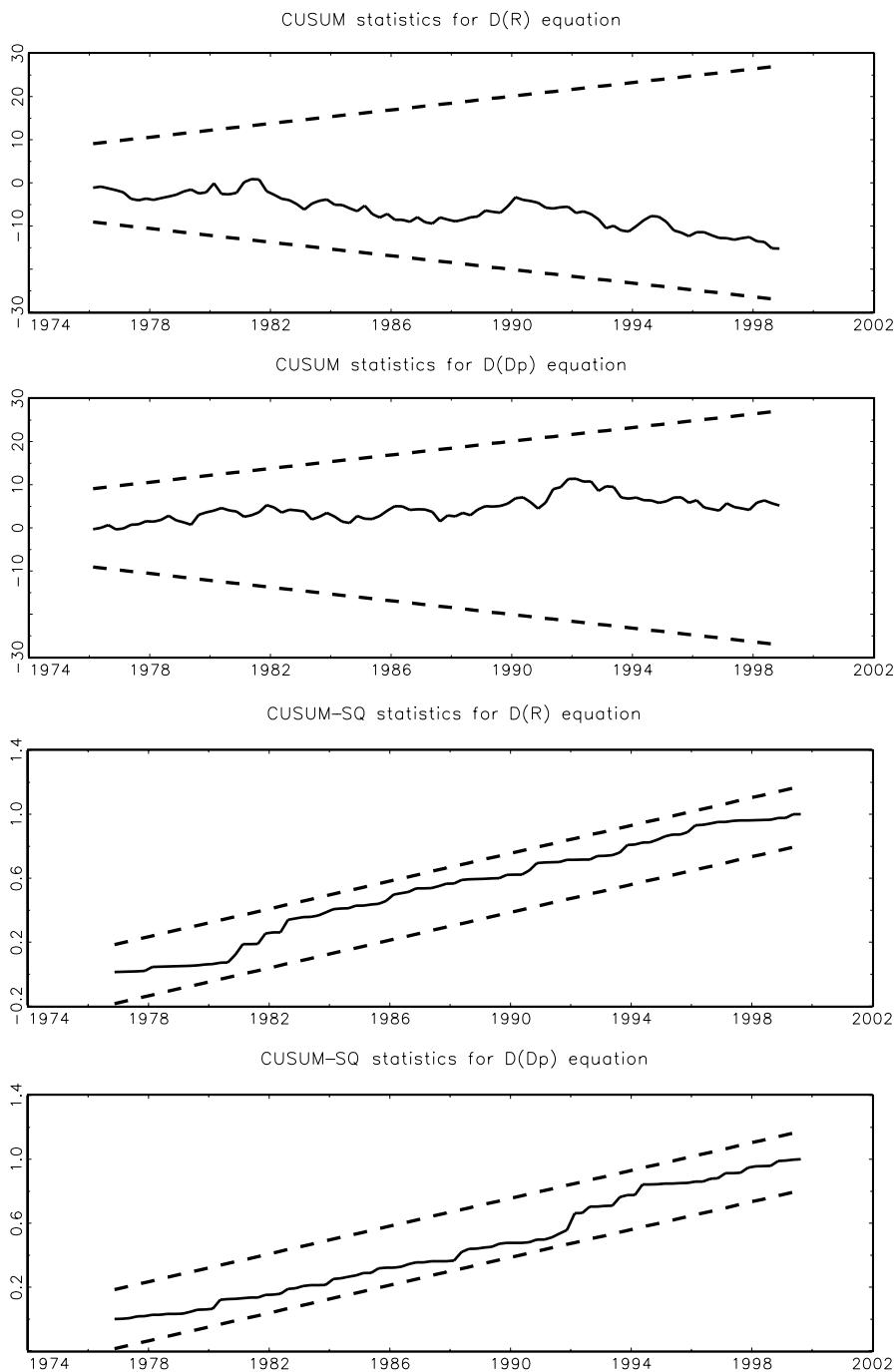
Figure 3.4. CUSUM and CUSUM-of-squares tests of subset VECM (3.41) for German interest rate–inflation system with 5% level critical bounds (sample period: 1973Q2–1998Q4).
