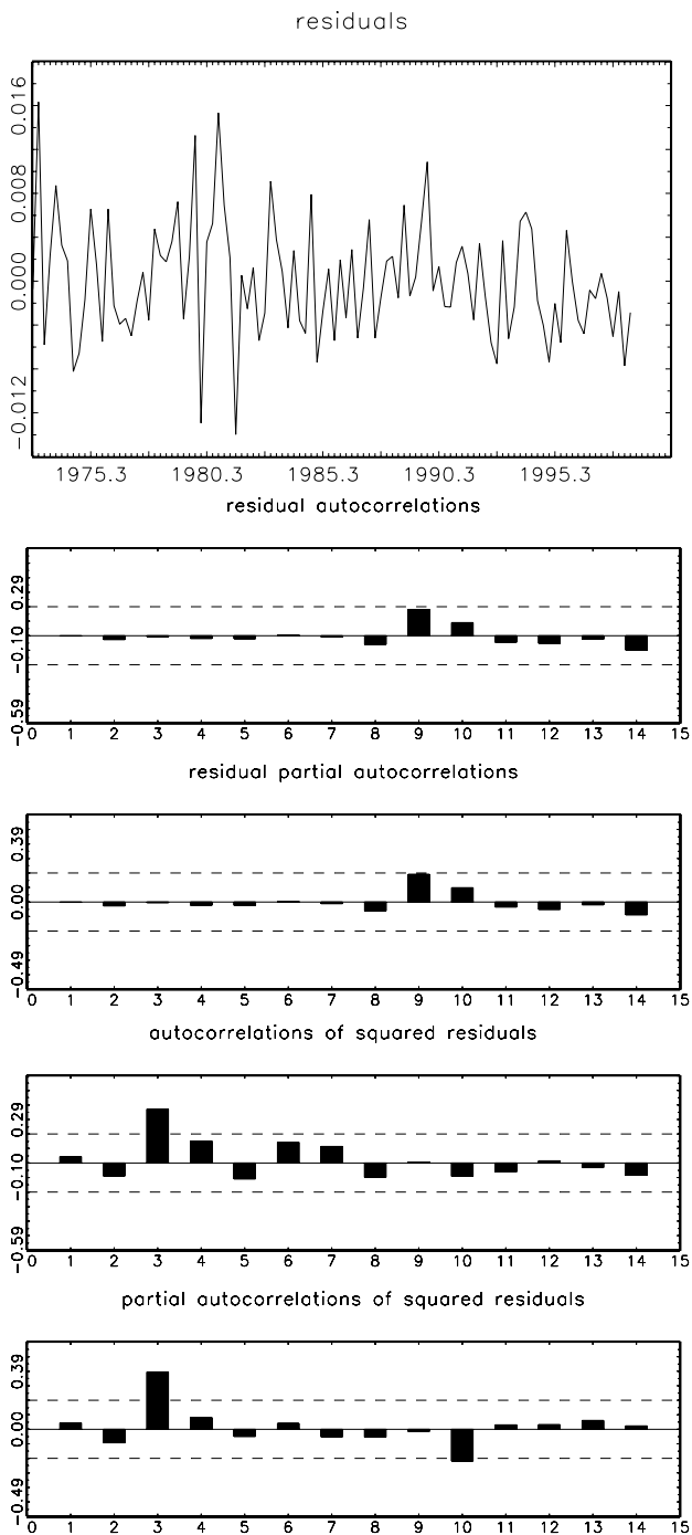
Figure 2.8. Plots of residuals from AR(4) model for German long-term interest rate, autocorrelations, and partial autocorrelations of residuals and squared residuals.
