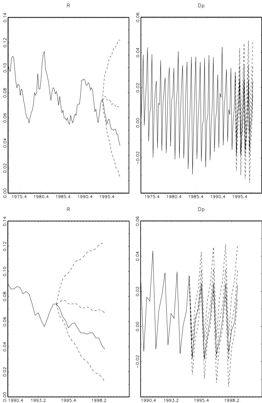
Figure 3.6. Forecasts of the German interest rate-inflation system with 95% forecast intervals based on subset VECM (3.41); estimation period: 1973Q2–1994Q4.
