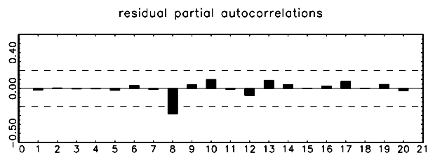
Figure 2.12. Diagnostics of AR(4) residuals of U.S. investment series.
