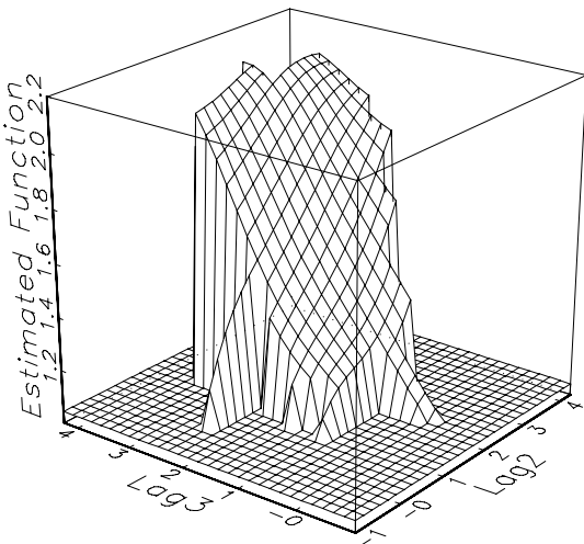
(b) All grid points for which the estimated density is within the 10%-quantile are removed and the data are standardized with standard deviation 0.0110
