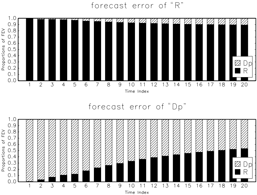
Figure 4.2. Forecast error variance decomposition of German interest rate–inflation system based on subset VECM (3.41).
